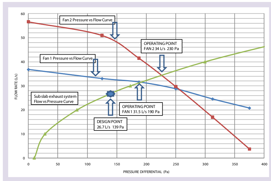
Figure 10 Fan Selection Graphical Solution
