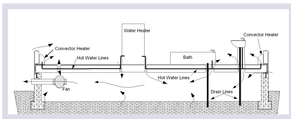
Figure I4 – Crawlspace Exhaust
