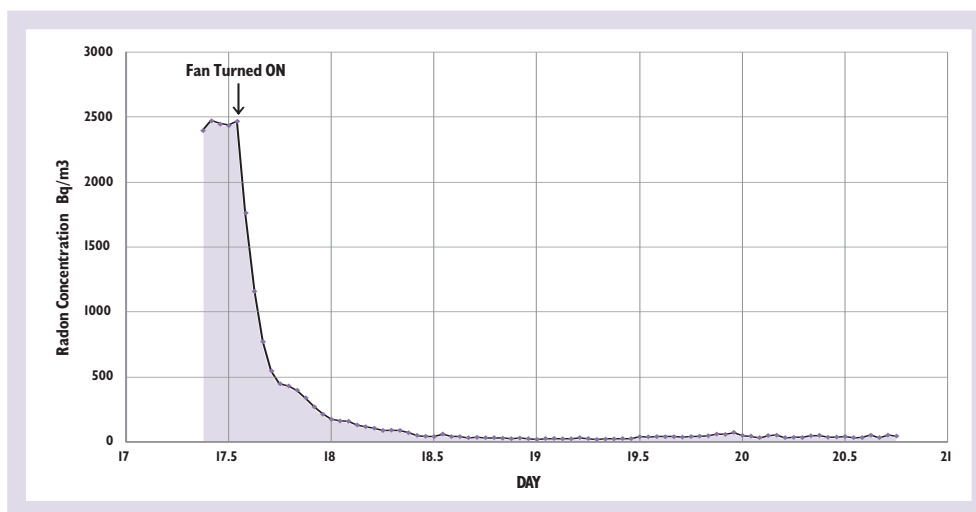
Figure 16 – Change in Radon Concentration after Mitigation (Data Courtesy of Health Canada)
