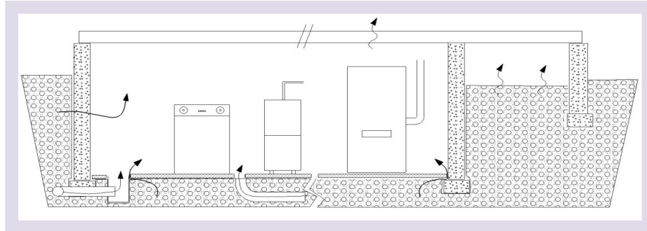
Figure 5 – Radon Entry Routes for a Poured Concrete Foundation
