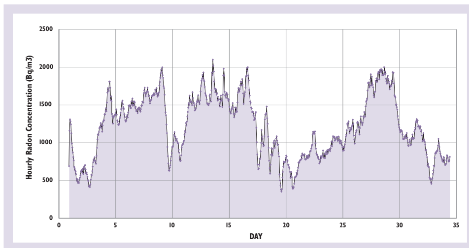
Figure 2 – Example of Radon Concentration Variability (Data courtesy of Health Canada)
