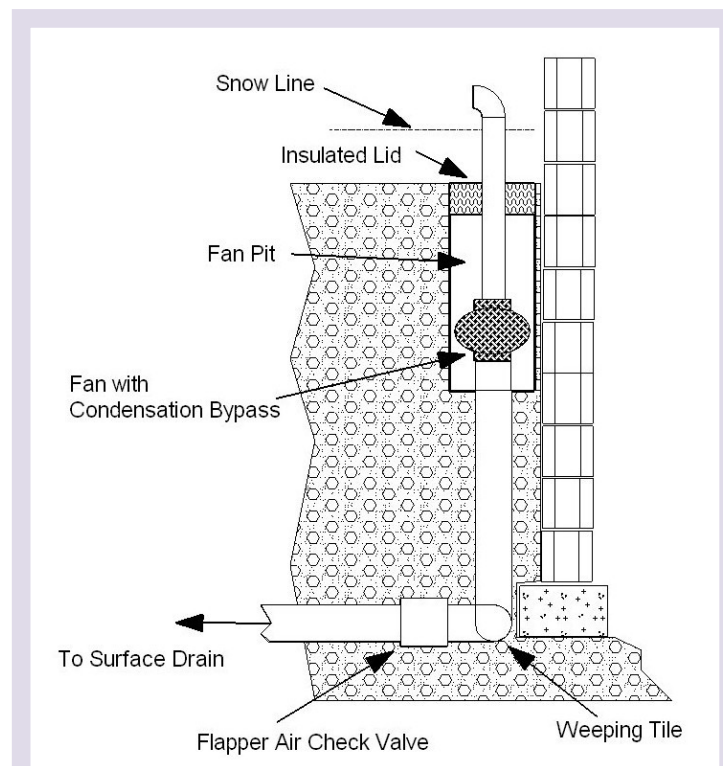
Figure I3 – Weeping tile Exhaust
