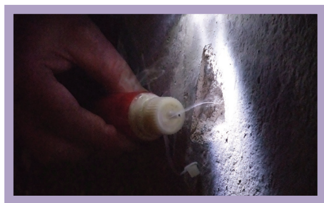
Picture 8 – Use of chemical smoke
