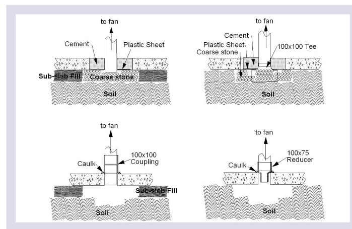
Figure 9 – Exhaust Pipe Connection Details
