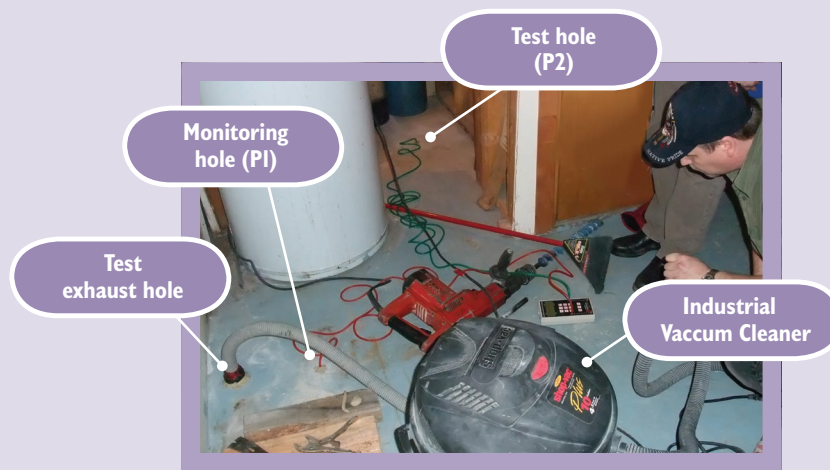
Picture 2 – Feasibility test installation
