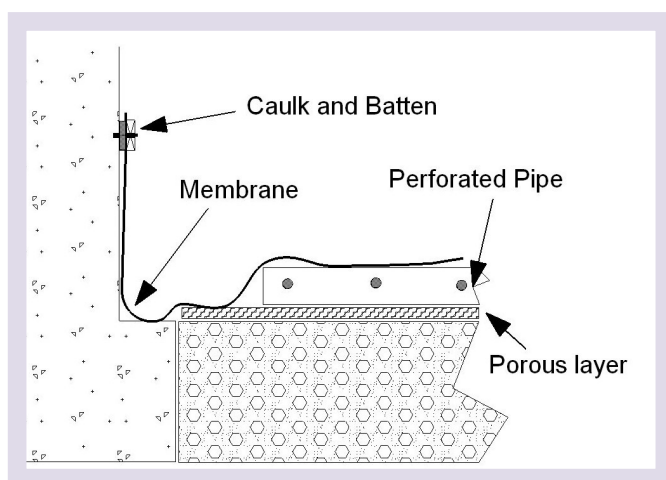
Figure 11 – Membrane and Wall Attachment
