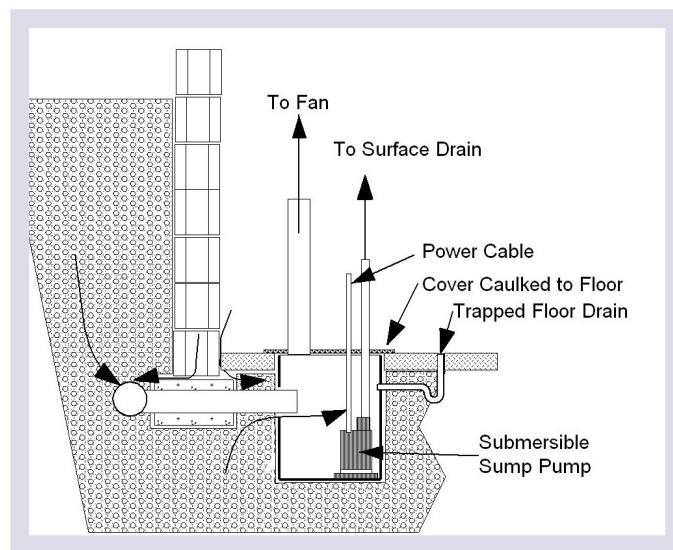
Figure I2 – Sump Exhaust
